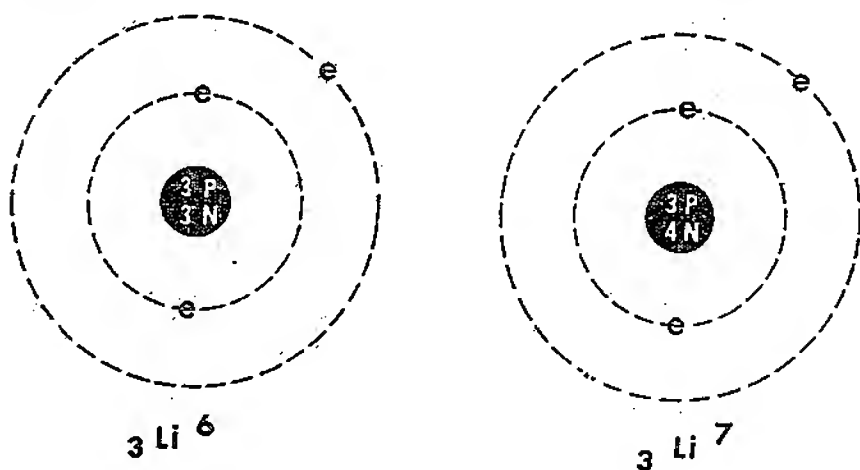
Figure 2—Diagram of Lithium Isotopes.
